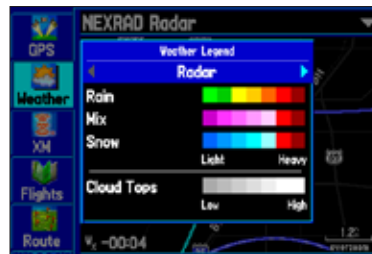
Weather Legend
