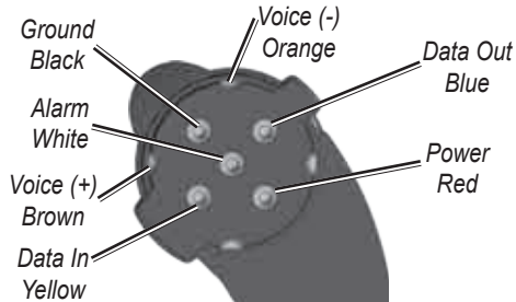
Power/Data Connector on the GPSMAP 396 Unit
